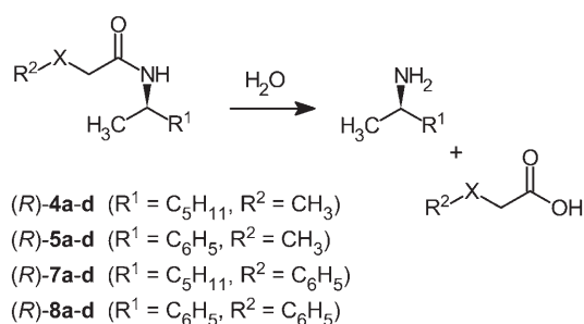
Figure 5. Hydrolysis of the enantiomerically pure amides 4 , 5 , 7 and 8 (full structures are given in Figure 2 and Figure 4).
