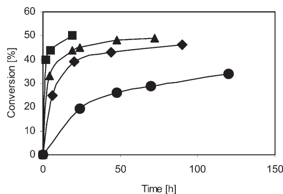
Figure 3. Effects of the acyl donor on the acylation of 2 ; ( \blacklozenge ) 3a , \text{X} = \text{NH} ; ( \blacksquare ), 3b , \text{X} = \text{O} ; ( \blacktriangle ), 3c , \text{X} = \text{S} ; ( \bullet ), 3d , \text{X} = \text{CH}_2 .
