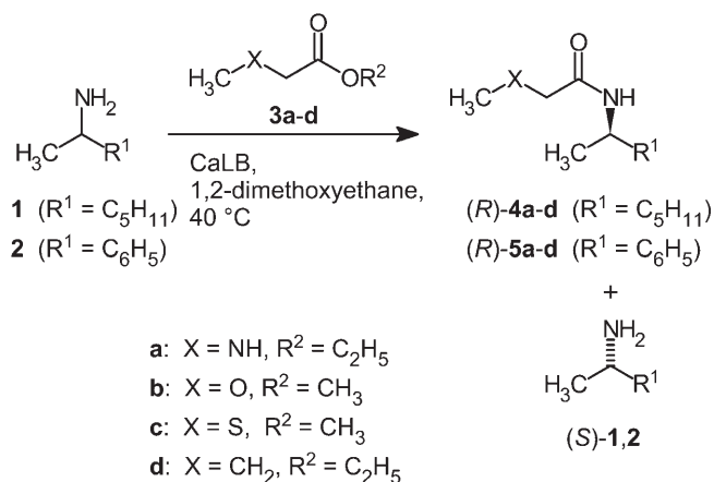
Figure 2. CaLB-catalyzed amine resolution with acyl reagents \text{CH}_3\text{-X-CH}_2\text{CO}_2\text{R}^2 .
