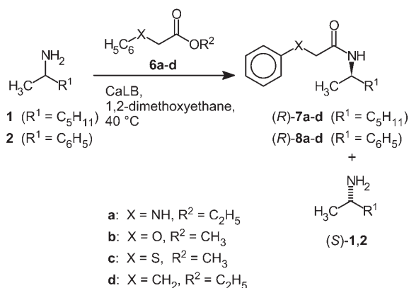
Figure 4. CaLB-catalyzed resolution with acyl reagents \text{C}_6\text{H}_5-\text{X}-\text{CH}_2\text{CO}_2\text{R}^2 .
