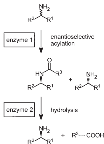
Figure 1. General scheme of fully enzymatic amine resolution.
